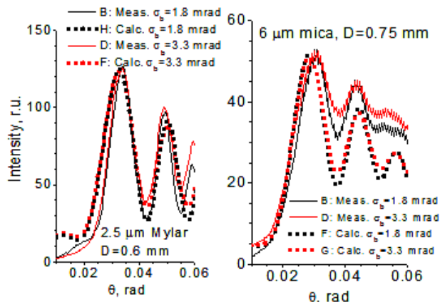
Figure 6: Measured (solid lines) and computed (dots) fringes for the Mylar (left) and mica (right) -based interferometers at normal incidence, beam energy of 16 MeV, \sigma_E \sim 100 keV and \sigma_{\text{meas}} = 0.9 mrad.
