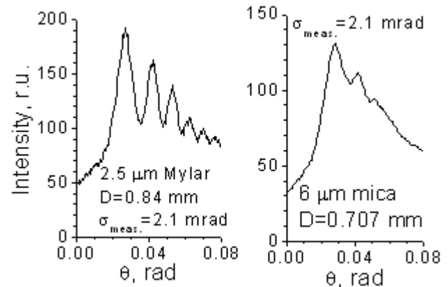
Figure 4: Fringe profiles obtained with Mylar-based (left) and mica-based (right) OTRI setup at 45° incidence and 16 MeV electrons and \sigma_b = 1.2 mrad.
